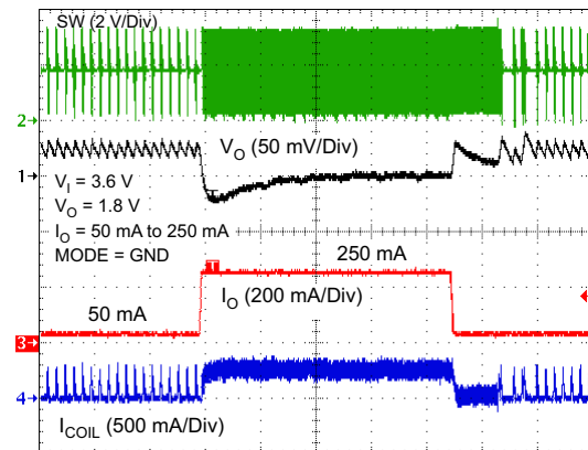
Figure 30. Load Transient (PFM Mode to PWM Mode)
