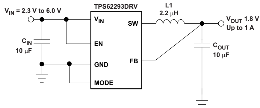
Figure 23. TPS62293DRV Fixed 1.8 V
