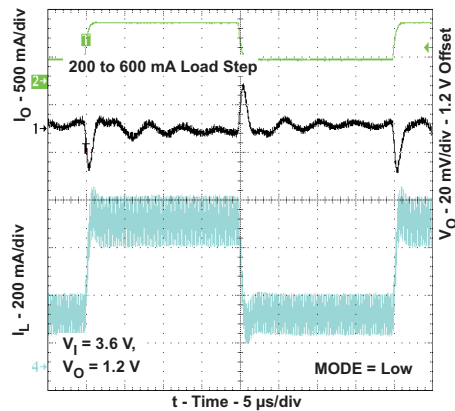
Figure 22. Load Transient Response in PFM/PWM Operation
