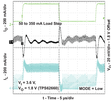
Figure 13. Load Transient Response in PFM/PWM Operation
