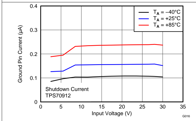
Figure 15. GND Current vs V_{IN} and Temperature
