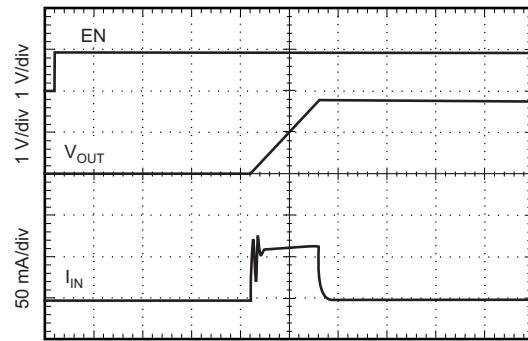
V_{\text{IN}} = 2.1 \text{ V} , V_{\text{OUT}} = 1.8 \text{ V} , I_{\text{OUT}} = 100 \mu\text{A}
