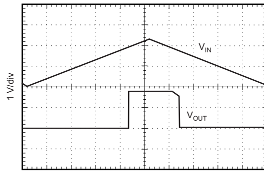
I_{\text{OUT}} = 200 \text{ mA}
