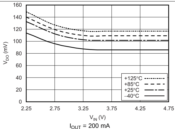
Figure 6. Dropout Voltage vs Input Voltage (TPS72750)
