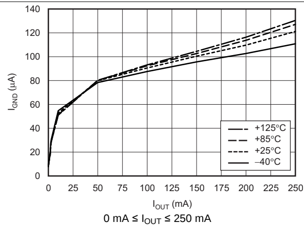
Figure 9. Ground Pin Current vs Load (TPS72718)
