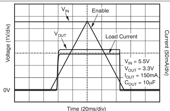
Figure 43. TPS780330220 Output Voltage vs Enable (Slow Ramp)
