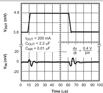
Figure 26. TPS79328 Line Transient Response
