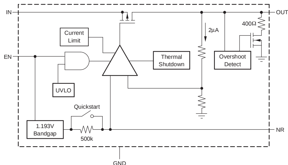
Figure 26. Fixed-Voltage Versions
