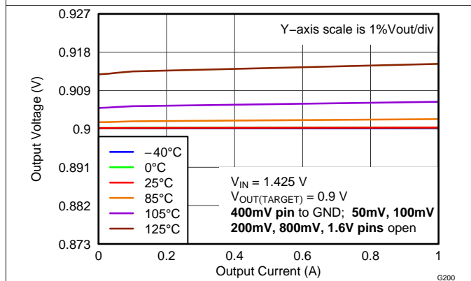
Figure 1. Load Regulation (0.9 V, Adjustable)
