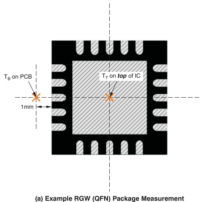
(a) Example RGW (QFN) Package Measurement
