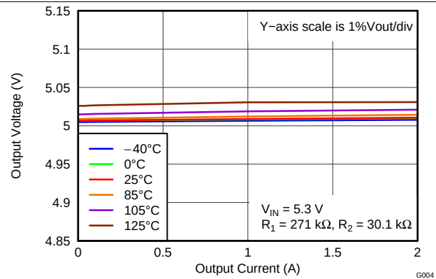
Figure 2. Load Regulation (5.0 V, Adjustable)
