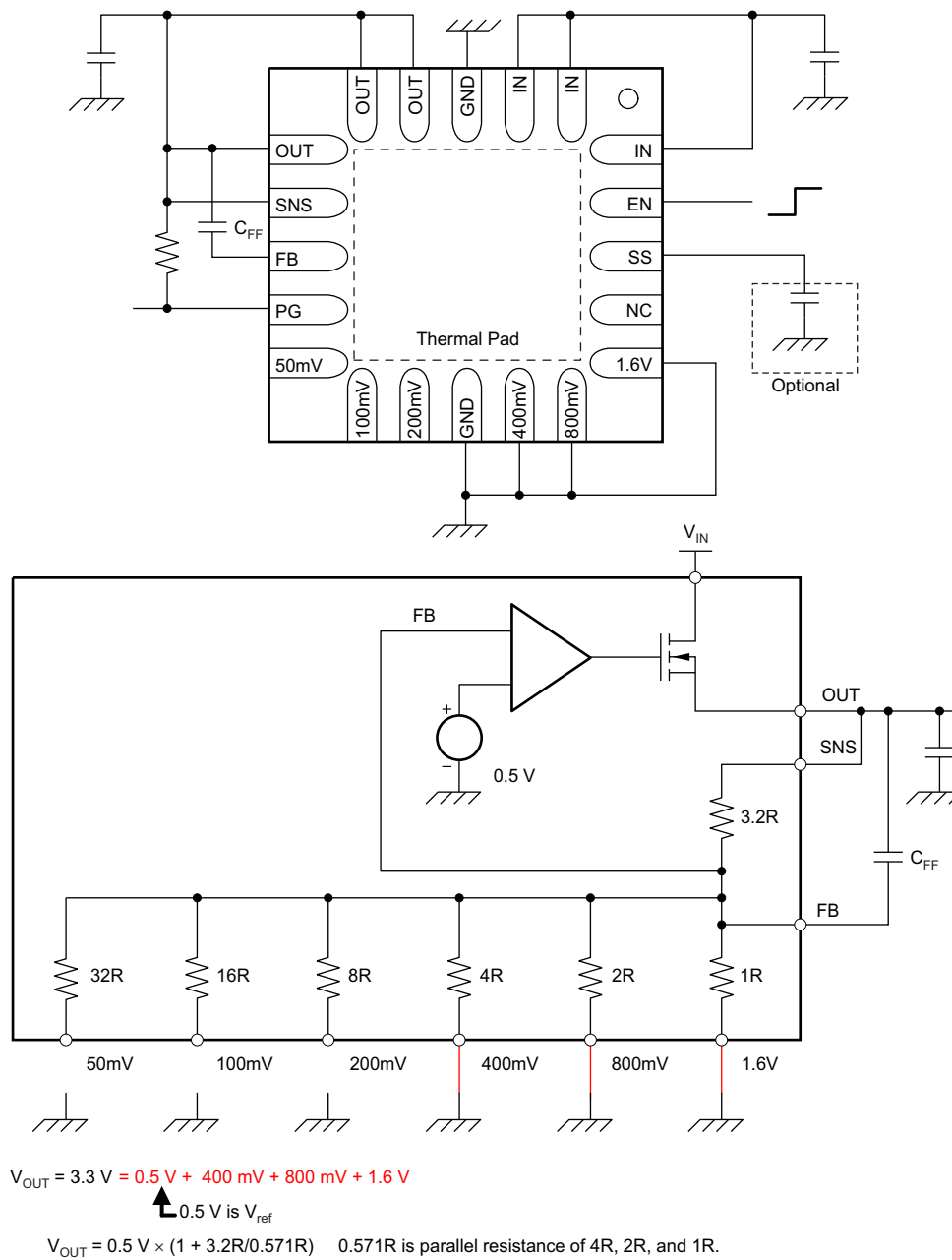
Figure 28. 3.3-V Configuration
