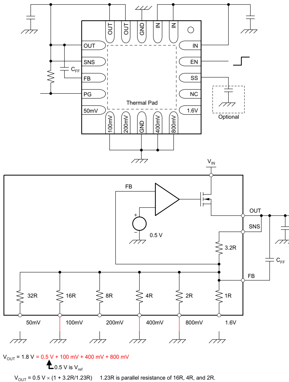
Figure 26. 1.8-V Configuration
