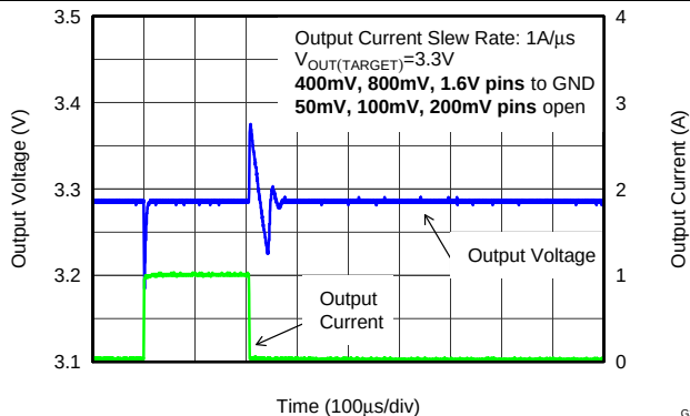
Figure 33. Load Transient Response ( V_{OUT} = 3.3\text{ V} )
