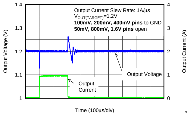
Figure 32. Load Transient Response ( V_{OUT} = 1.2\text{ V} )
