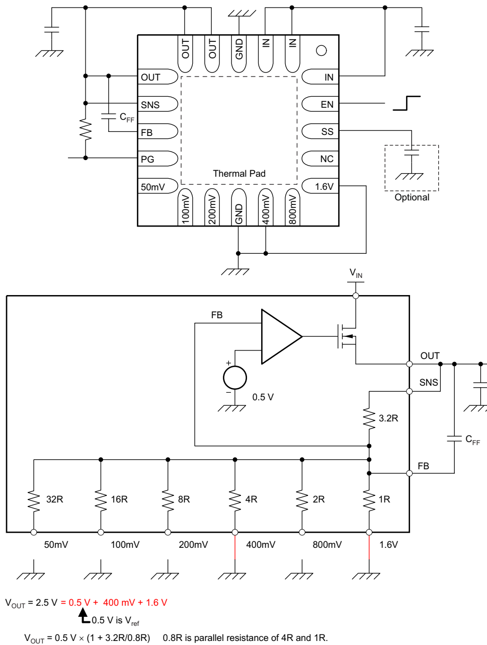
Figure 27. 2.5-V Configuration
