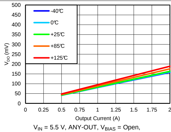
Figure 13. Dropout Voltage vs Output Current
