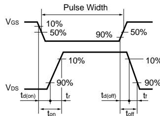
Fig.3-2 Switching Waveforms
