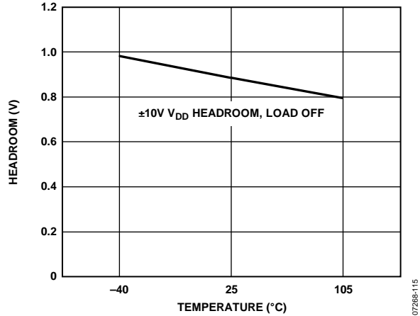
Figure 15. V_{DD} Headroom, \pm 10V Range, Output Set to 10V, Load Off
