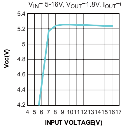
Vcc Regulator Line Regulation
