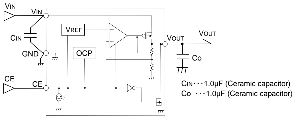
Figure 2. Block Diagrams
