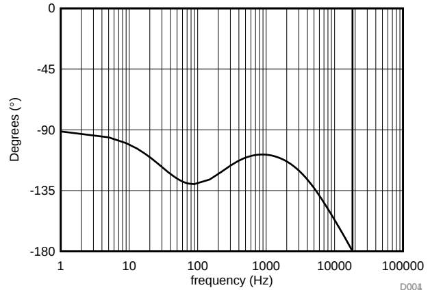
Figure 35. Converter Closed-Loop Bode Plot – Phase
