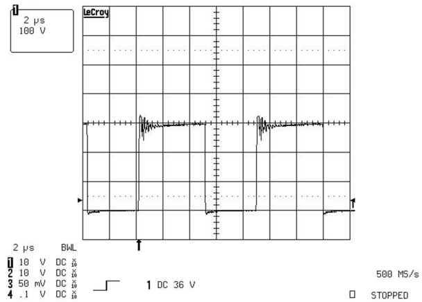
Figure 37. Primary Side MOSFET Drain to Source Voltage at 120-V AC Input (100 V/div)
