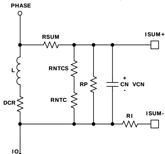
FIGURE 10. DCR CURRENT-SENSING NETWORK
