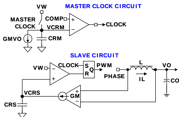
FIGURE 3. R 3 ™ MODULATOR CIRCUIT
