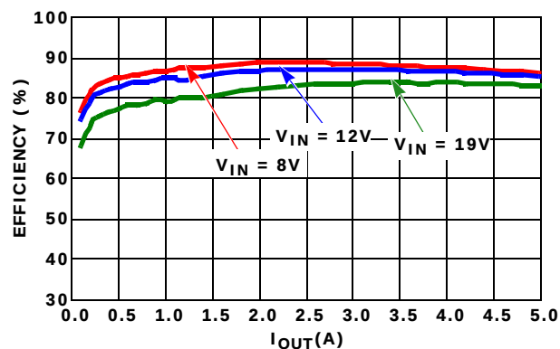
FIGURE 24. ISL62884CEVAL2Z EVALUATION BOARD DE MODE EFFICIENCY, V_{ID} = 1.2375V , V_{IN1} = 8V , V_{IN2} = 12.6V AND V_{IN3} = 19V
