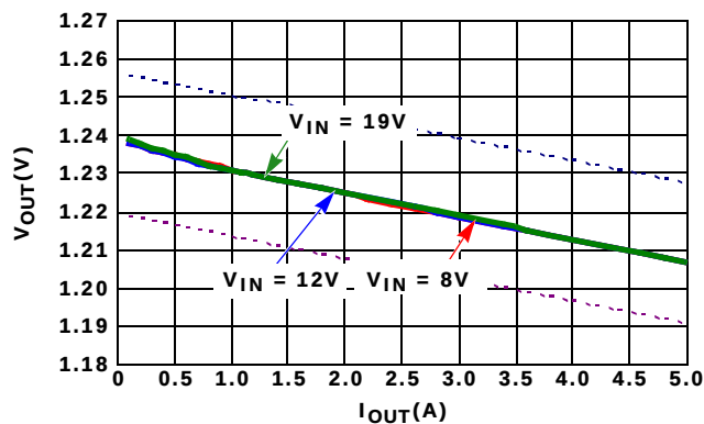
FIGURE 26. ISL62884CEVAL2Z EVALUATION BOARD DE MODE LOAD LINE, V_{ID} = 1.2375V , V_{IN1} = 8V , V_{IN2} = 12.6V AND V_{IN3} = 19V
