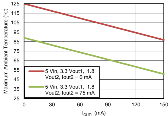
Figure 28. Maximum Ambient Temperature vs Output Current ( V_{IN} = 5\text{ V} , V_{OUT1} = 3.3\text{ V} , V_{OUT2} = 1.8\text{ V} )
