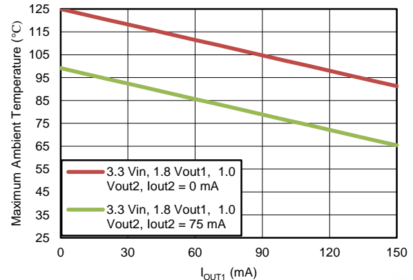
Figure 29. Maximum Ambient Temperature vs Output Current ( V_{IN} = 3.3\text{ V} , V_{OUT1} = 1.8\text{ V} , V_{OUT2} = 1\text{ V} )
