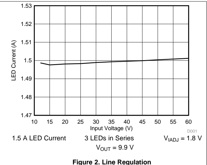
Figure 2. Line Regulation
