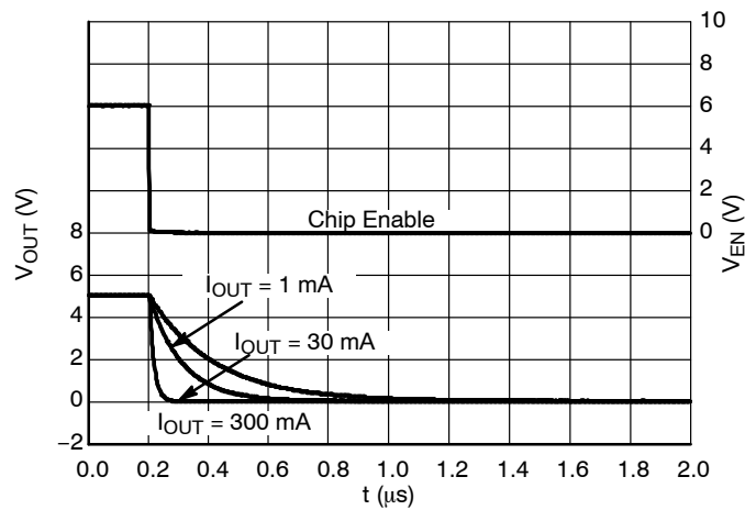
Figure 40. Shutdown, 5.0 V Version D, V_{IN} = 6.0 \text{ V}
