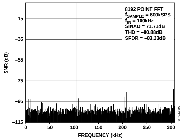
Figure 5. AD7476 Dynamic Performance at 600 kSPS
