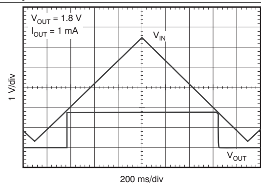
Figure 20. V_{IN} Ramp Up, Ramp Down Response
