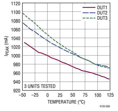
Typical R_{SNS} Current Limit vs Temperature
