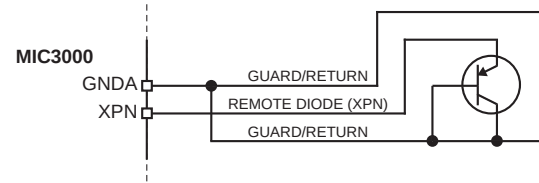
Figure 34. Guard Traces and Kelvin Return for Remote Thermal Diode
