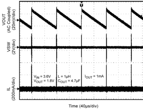
Switching Waveform
