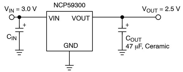
Figure 2. Fixed 2.5 V Regulator in D²PAK-3 Package
