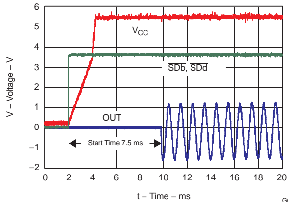
Figure 30. Start-Up Time
