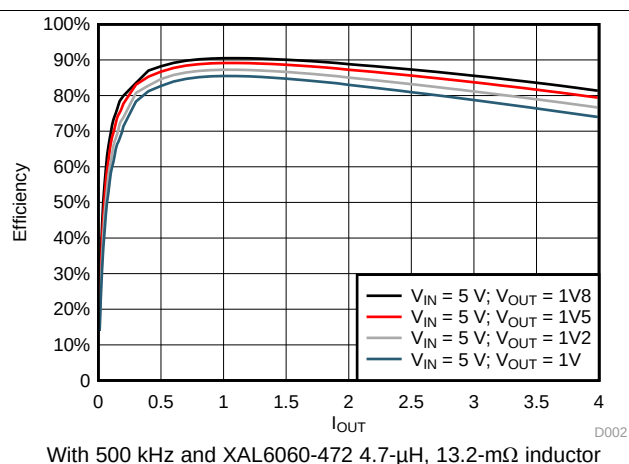
Figure 2. Buck1 and Buck2 Power Efficiency, V_{IN} = 5\text{ V}
