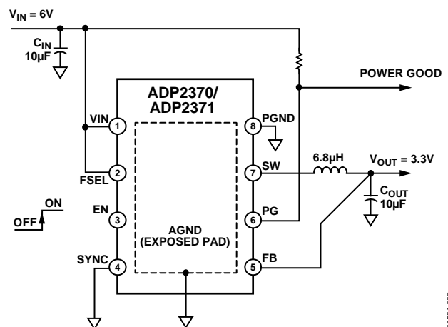
Figure 82. Typical Application, 1.2 MHz, Fixed Output
