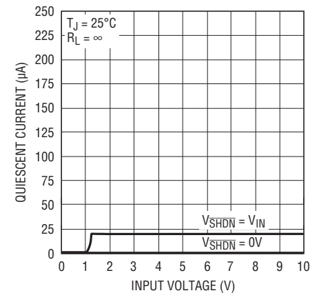
LT1761-1.2 Quiescent Current
