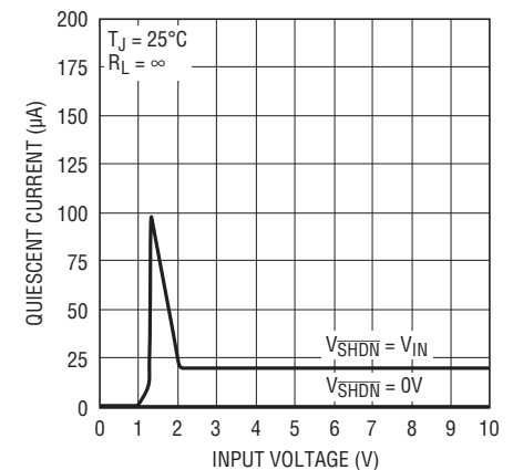
LT1761-2 Quiescent Current
