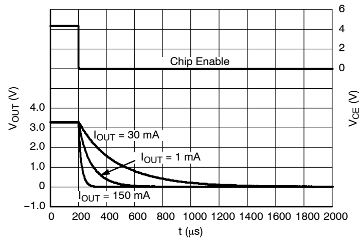
Figure 37. Shutdown, 3.3 V Version D, V_{IN} = 4.3 V
