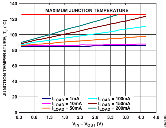
Figure 57. WLCSP, T_A = 85^\circ\text{C}
