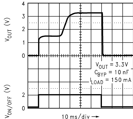
Figure 38. Turnon Time
