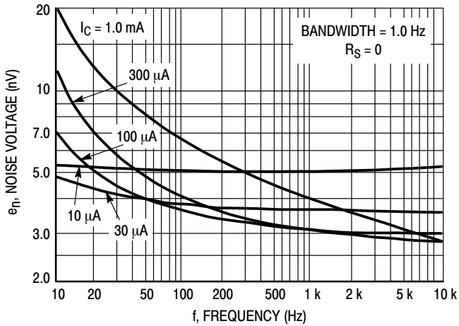
Figure 4. Noise Voltage
