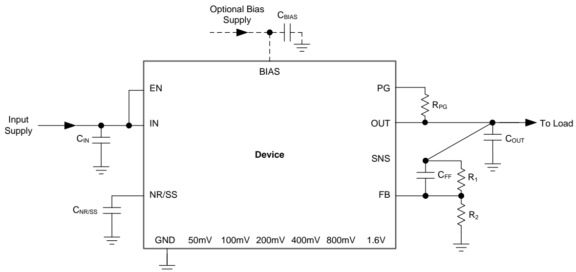
Figure 45. Adjustable Operation
