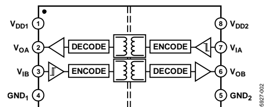
Figure 2. ADuM3201 Functional Block Diagram
