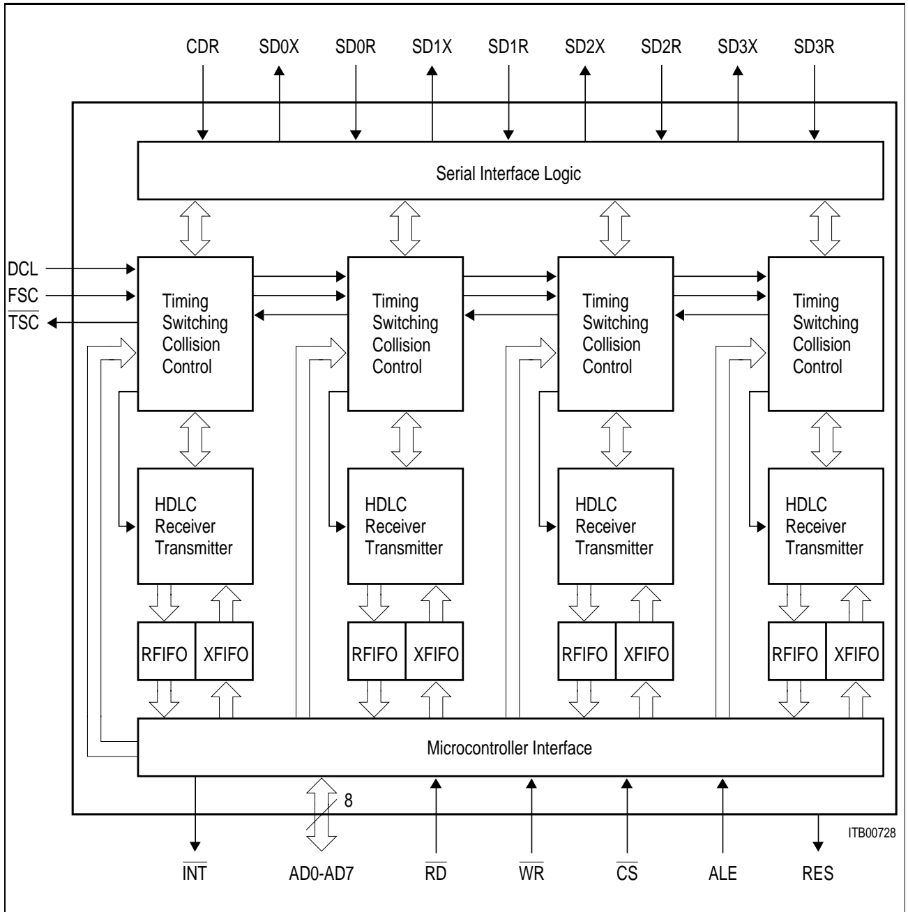
Block Diagram
