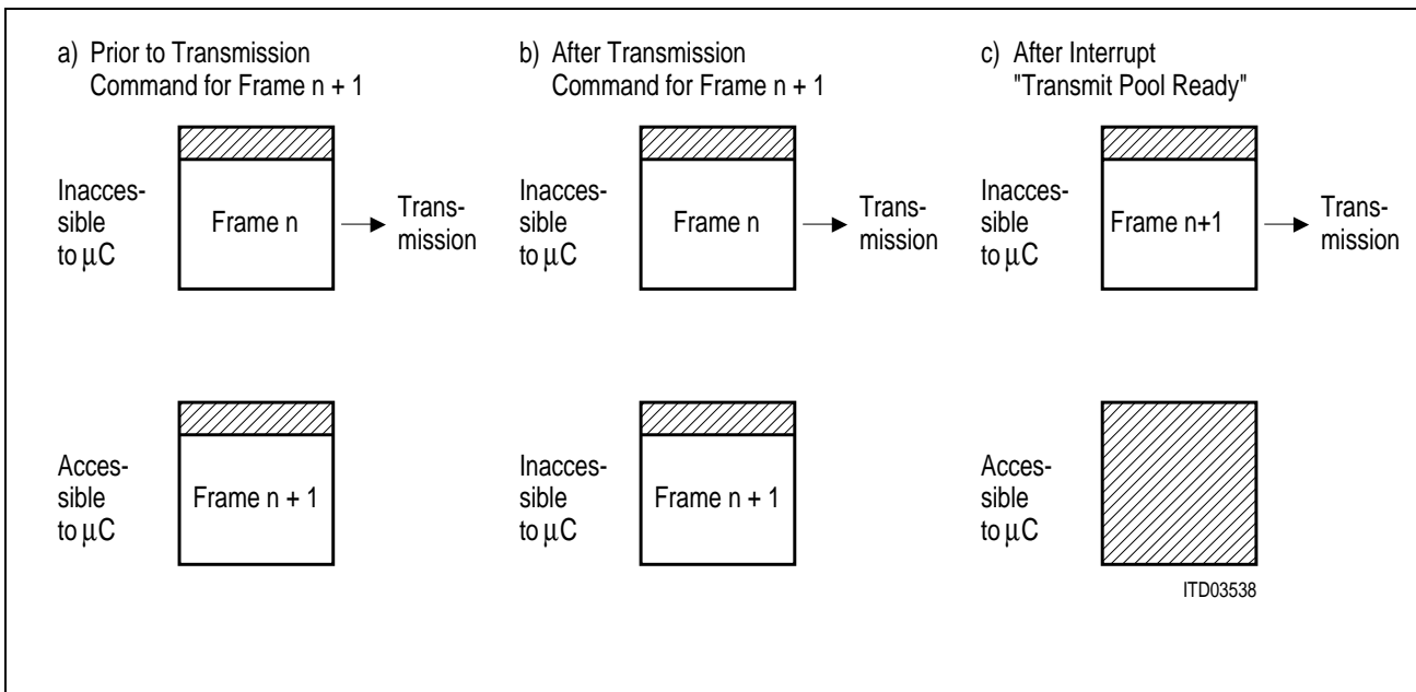
Figure 11 Transmit FIFO
