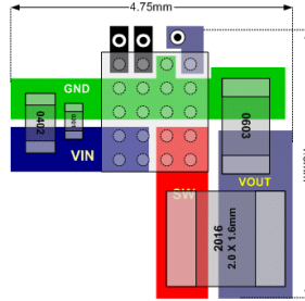
Figure 2. Reduced-Footprint Layout
