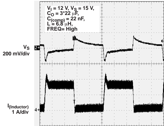
100 \mu\text{s}/\text{div} Figure 6.
