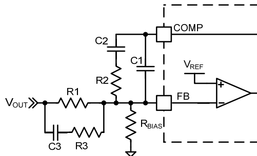
Figure 33. Compensation Network
