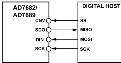
FOR SPI USE CPHA = 0, CPOL = 0.
