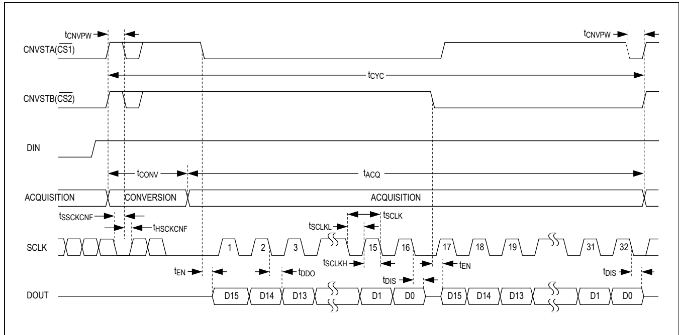
Figure 11. Multichannel \overline{\text{CS}} Configuration Timing
