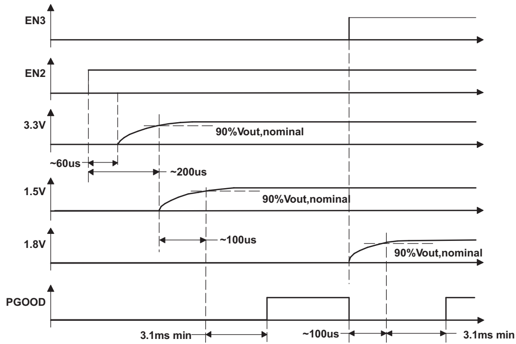
Figure 6. Timing Diagram
