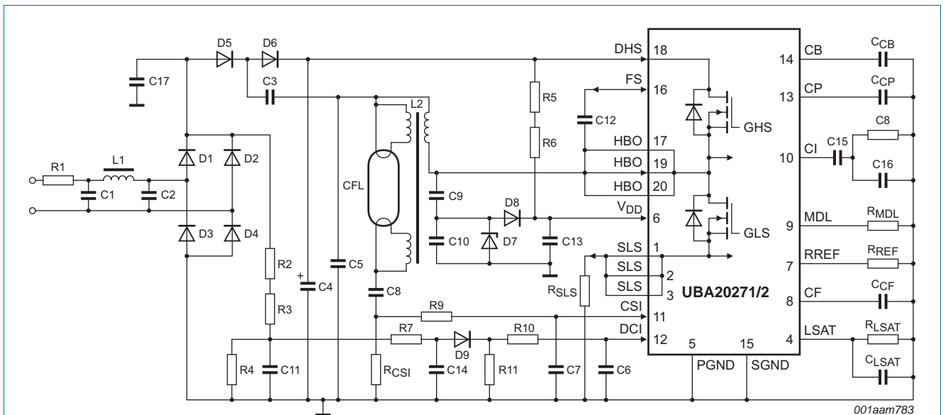
Fig 11. Application diagram
