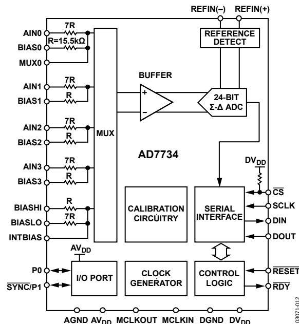
Figure 12. Block Diagram
