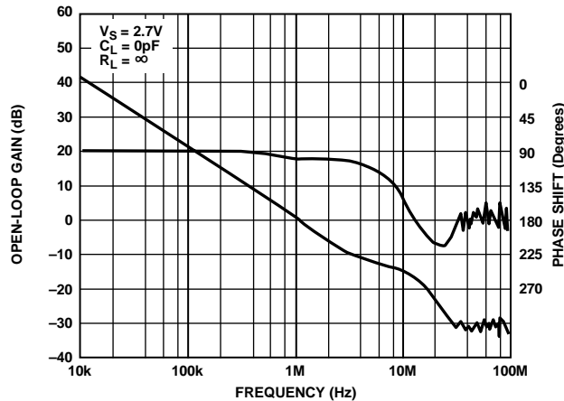
Figure 17. Open-Loop Gain and Phase Shift vs. Frequency
