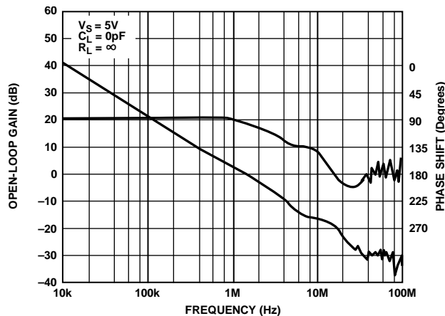
Figure 18. Open-Loop Gain and Phase Shift vs. Frequency
