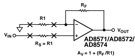
Figure 55. Using Dummy Components to Cancel Thermoelectric Voltage Errors
