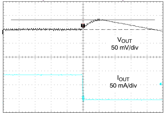
Figure 24. 100 mA to 10 mA Load Transient ( V_{IN} = 3.6\text{ V} , V_{OUT} = 1.2\text{ V} , T_A = 25^\circ\text{C} )
