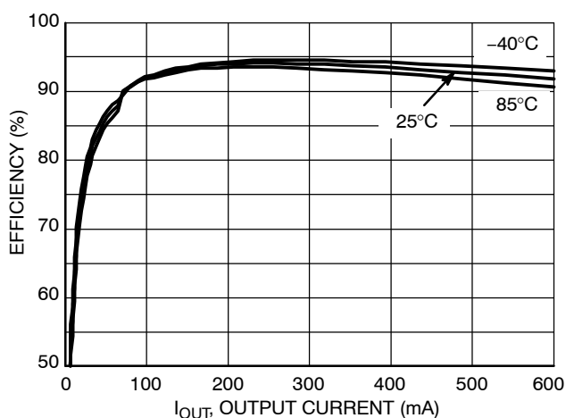
Figure 29. Efficiency vs. Output Current ( V_{IN} = 5.0 V, V_{OUT} = 3.9 V)
